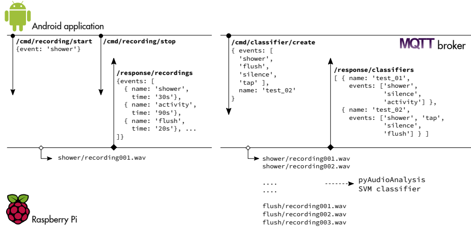
Fig. 1. From left to right: User initiates an event recording and the corresponding file is created. When user stops, a response is returned with information about the events recorded so far. When a reasonable amount of data is gathered, an SVM classifier for the desired events can be created using the pyAudioAnalysis library. In this case, the response contains information about the classifiers available for future use.
